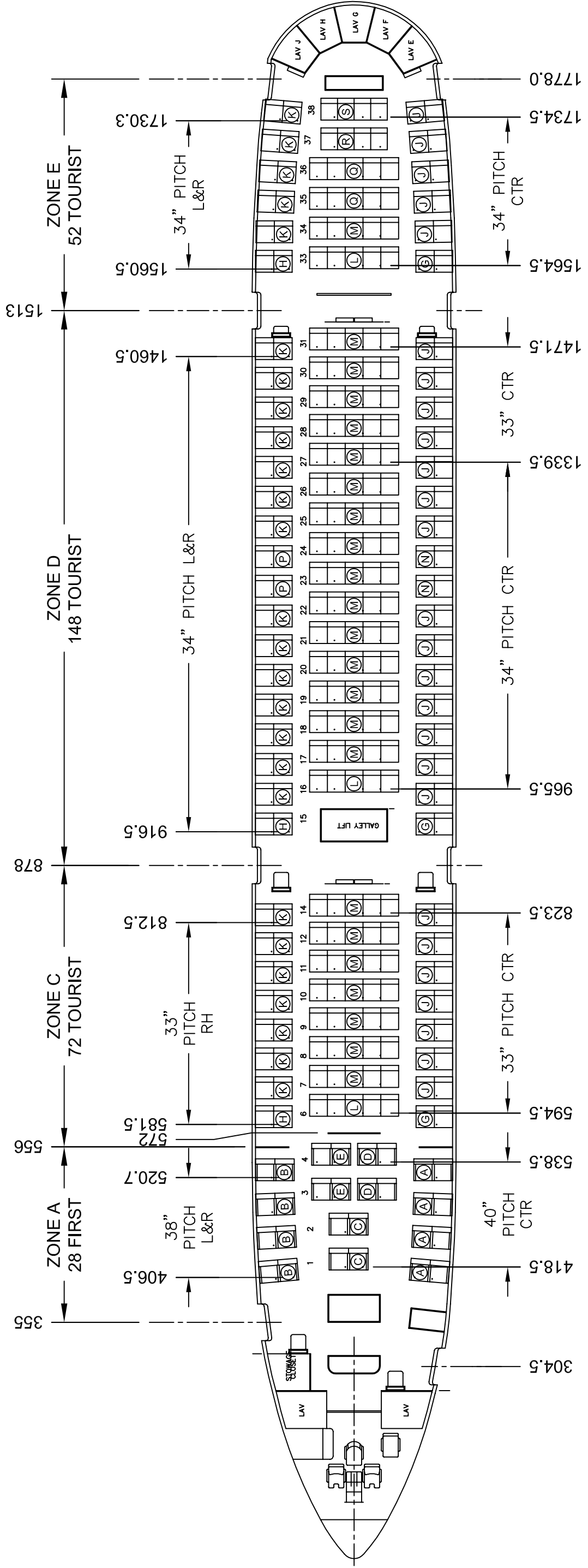
300 PAX CONFIGURATION 28 FIRST CLASS / 272 ECONOMY
